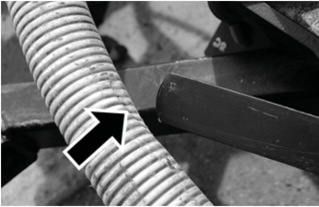
Figure 19. Damage to Primary Distribution Hose.
