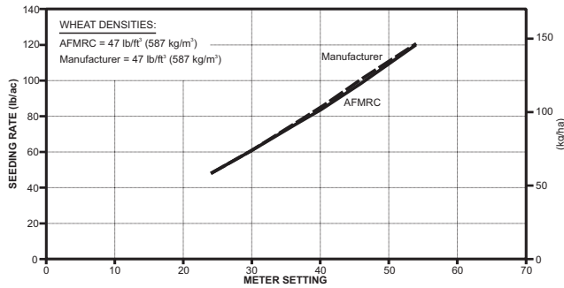
Figure 4. Metering Accuracy in Wheat.
