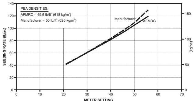
Figure 6. Metering Accuracy in Peas.
