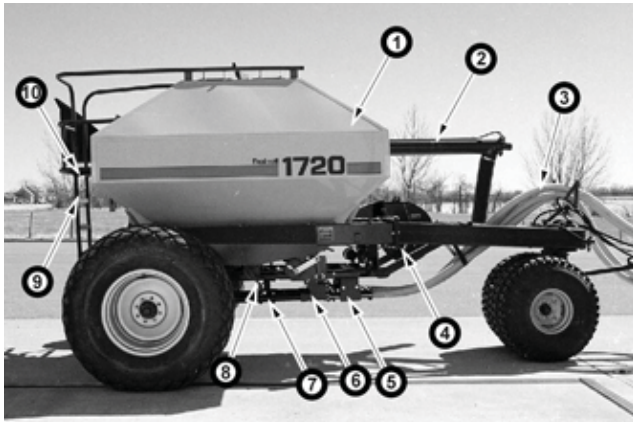
Figure 1. Flexi-coil 1720 Air Cart (1) Tank (2) Auger (3) Primary Hose (4) Centrifugal Fan (5) Centre Manifold (6) Metering Drive System (7) Intermediate Manifold (8) Hand Crank (9) Ladder and (10) Rear Platform.
