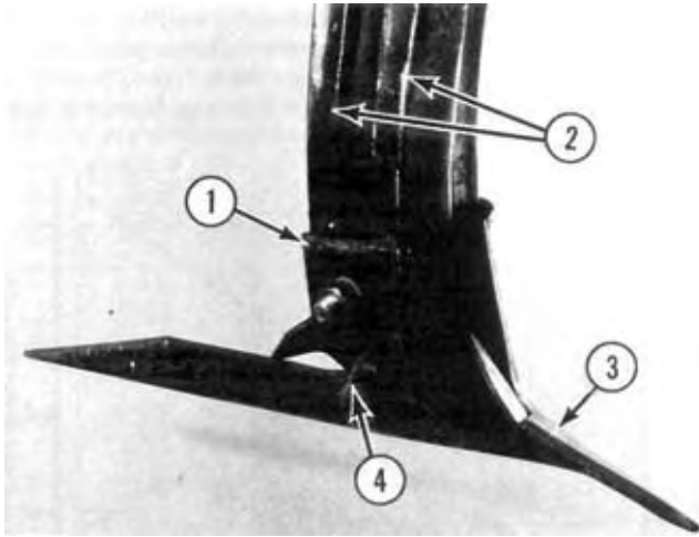
FIGURE 12. John Shearer Seed Boot: (1) Seed Boot, (2) Secondary Outlet Tubes, (3) Sweep, (4) V-shaped Spreader.
