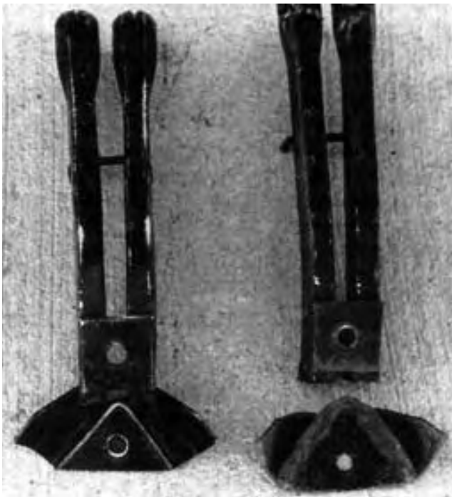
FIGURE 21. Seed Boot Failure.
