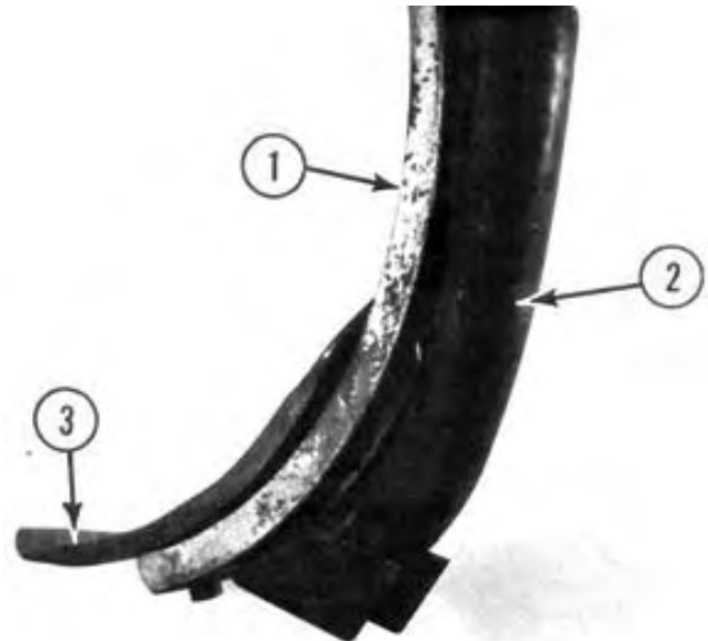
FIGURE 16. John Shearer Banding Boot: (1) Cultivator Shank, (2) Banding Boot, (3) Chisel Point.
