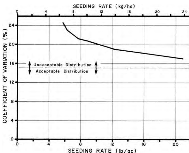
FIGURE 10. Distribution Uniformity in Canola Over a Range of Seeding Rates at 5.5 mph (9 km/h).
