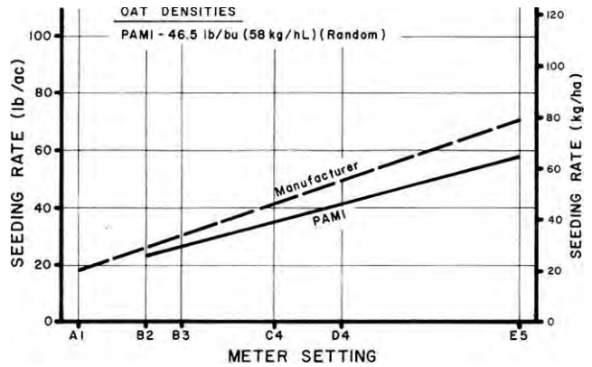
FIGURE 4. Metering Accuracy in Oats Using a Calibration Chart Multiplication Factor of 1.
