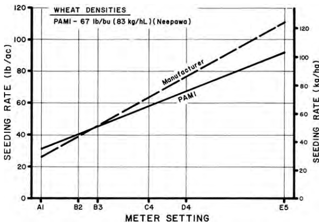
FIGURE 2. Metering Accuracy in Wheat Using a Calibration Chart Multiplication Factor of 1.
