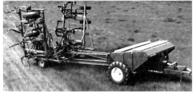
FIGURE 17. Transport Position.
