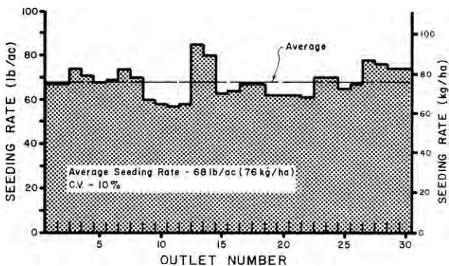
FIGURE 8. Distribution Uniformity Pattern in Wheat at 68 lb/ac (76 kg/ha).
