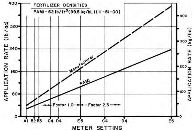
FIGURE 5. Metering Accuracy in Fertilizer Using a Calibration Chart Multiplication Factor of 1 and 2.3.
