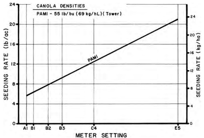
FIGURE 6. PAMI's Meter Calibration Curve in Canola Using the Low Range Sprocket Combination.
