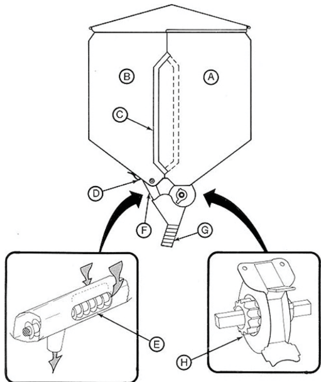
FIGURE 7. Seed and Fertilizer Metering System: (A) Grain Box, (B) Fertilizer Box, (C) Two Position Box Partition, (D) Fertilizer Cleanout Panel, (E) Fertilizer Auger, (F) Fertilizer Spout, (G) Grain and Fertilizer Drop Tube, (H) Externally Fluted Feedroll.
