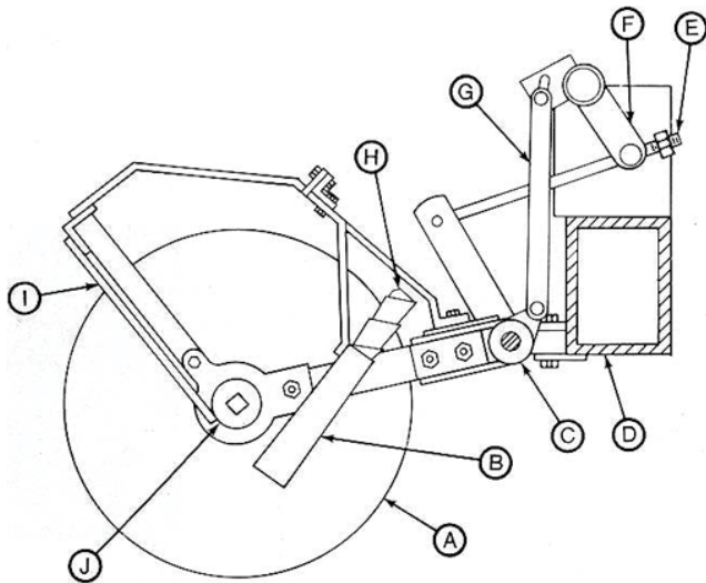
FIGURE 2. Disk Gang: (A) Disk, (B) Seed Spout, (C) Torsion Bar, (D) Main Frame, (E) Lift Rod, (F) Lift Arm, (G) Torsion Bar Linkage, (H) Coiled Seed Tube, (I) Trash Guard, (J) Gang Bearing.
