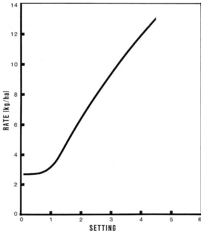
FIGURE 10. Alfalfa Calibration Using the Extra Slow Speed Drive and Seed Cup Filler Plates. Grain Density – 712 kg/m 3 (57 lb/bu).
