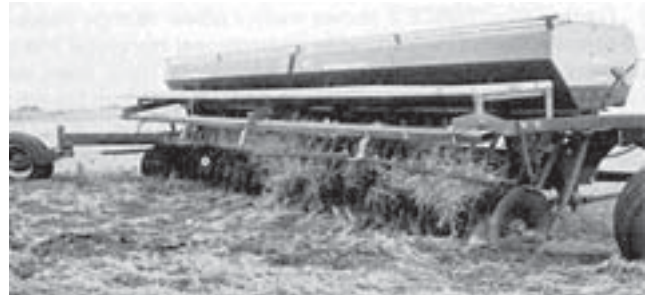
FIGURE 19. Uneven Penetration in Hard Soils Due to Improper Adjustment of Disk Gang Springs.
