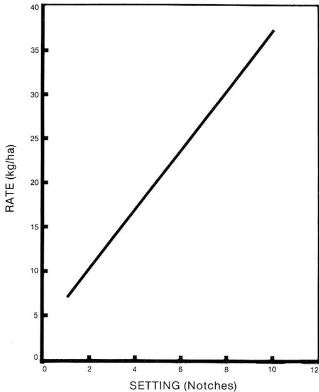
FIGURE 12. Alfalfa Calibration Using the Low Speed Drive Grain Density - 719 kg/m 3 (56 lb/bu).
