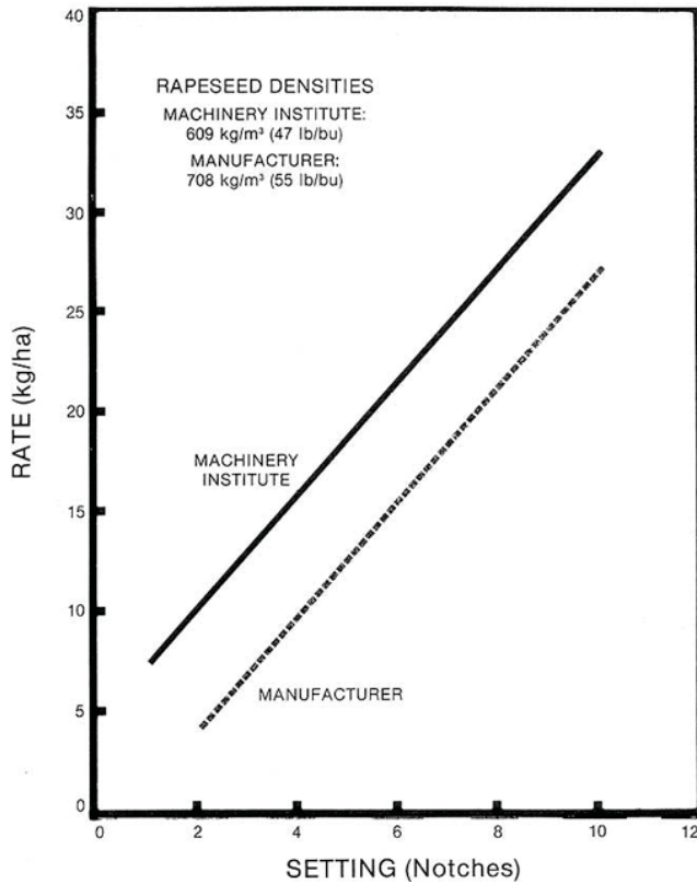
FIGURE 9. Rapeseed Calibration Using the Low Speed Drive.
