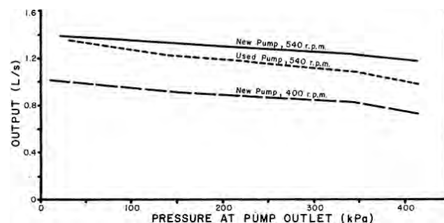
FIGURE 11. Pump Curves.
