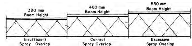
FIGURE 9. The Effect of Boom Lift and Drop on Spray Overlap.
