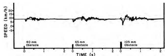
FIGURE 10. Typical Variation in Boom End Speed when the Boom Wheels are Driven over Different Obstacles at an Average Forward Speed of 9 km/h (5.6 mph).
