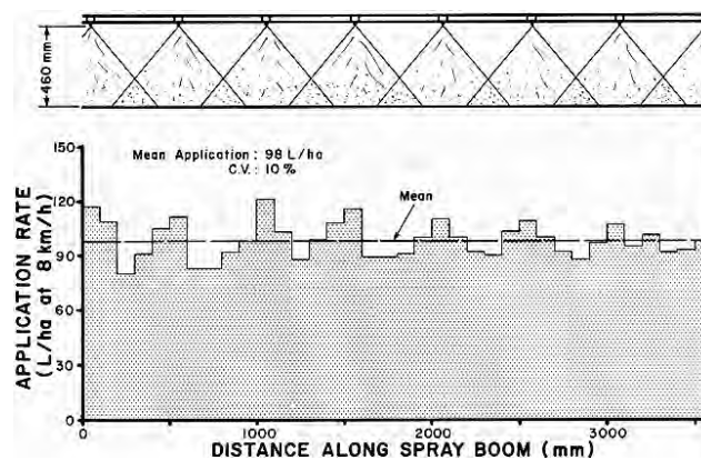
FIGURE 3. Typical Distribution Pattern along the Boom at 275 kPa (40 psi) with Tee Jet 8002 (80°) nozzles, at a 460 mm (18 in) Nozzle Height.
