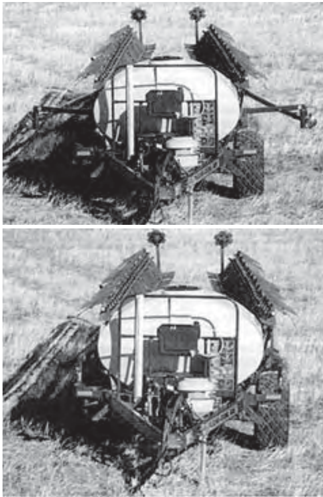
Figure 11. Flexi-coil sprayer in transport position. Top: Field Transport, Bottom: Road Transport.
