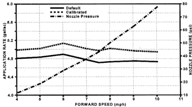
Figure 2. Application rate and nozzle pressure at various speeds with the controller programmed to apply 5 gal/ac (55 L/ha).
