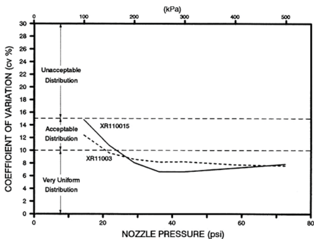
FIGURE 7. Spray Pattern Uniformity for Spraying Systems Extended Range TeeJet XR110015VS and XR11003VS Stainless Steel Nozzles Operated at a 15 in (381 mm) Nozzle Height and 30 Degree Forward Spray Angle.
