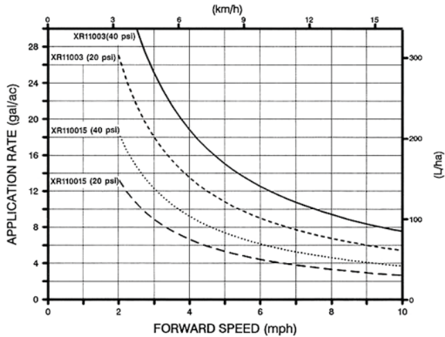
FIGURE 2. Application Rates at Various Forward Speeds and Pressures Using Spraying Systems Extended Range Tee Jet XR110015VS and XR11003VS Nozzles.
