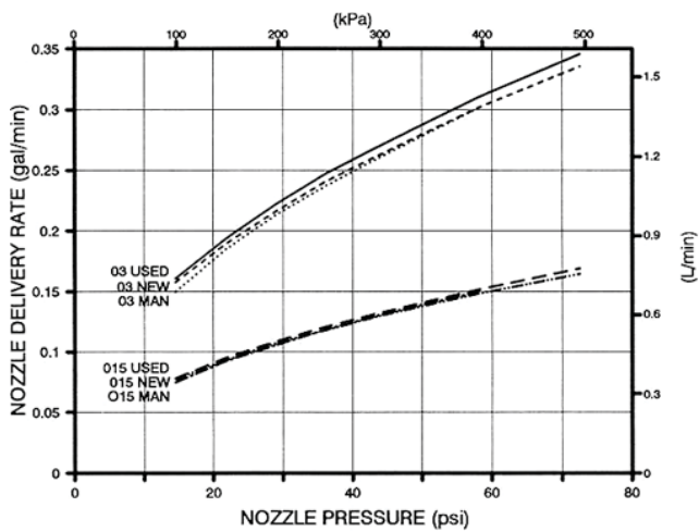
FIGURE 3. Delivery Rates for Spraying Systems Extended Range Tee Jet XR110015VS and XR11003VS Stainless Steel Nozzle Tips.
