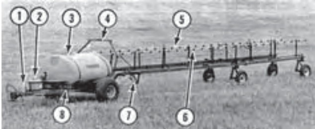
FIGURE 1. Harmon Model 833 Auto-Fold Field Sprayer: (1) Hydraulic Motor and Pump, (2) Easy-Fill Chemical Tank, (3) Spray Tank, (4) Auto-fold Overhead Bar, (5) Spray Boom, (6) Nozzle Body Assembly, (7) Nozzle Height Adjustment Ram and (8) Reload, Agitation Solenoid Valves.
