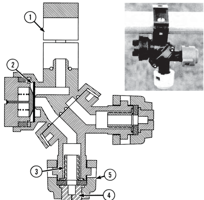
FIGURE 9. Swivel-Jet Diaphragm Dual Nozzle Body Assembly: (1) Split-Eyelet Clamp, (2) Diaphragm Check Valve, (3) Strainer, (4) Nozzle Tips, and (5) Quick-Disconnect and Self-Aligning Nozzle Cap.
