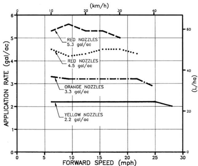
FIGURE 2. Application Rates at Various Forward Speeds Using Albus Nozzles.
