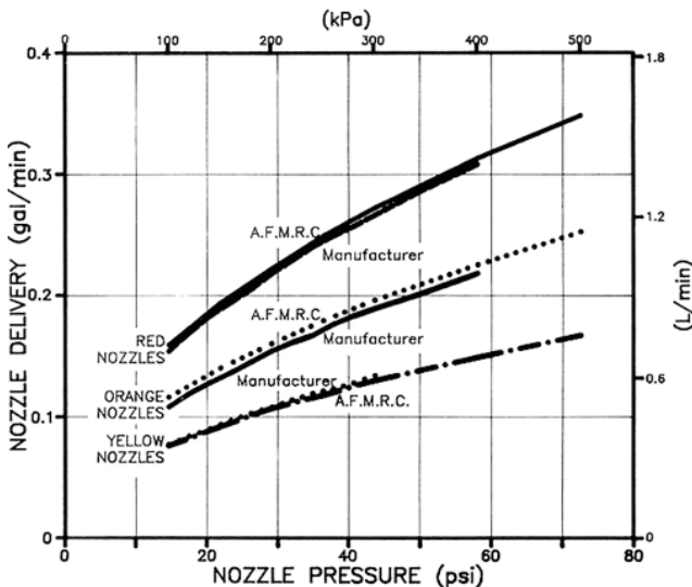
FIGURE 5. Delivery Rates for Albus Yellow, Orange and Red Ceramic Nozzle Tips.
