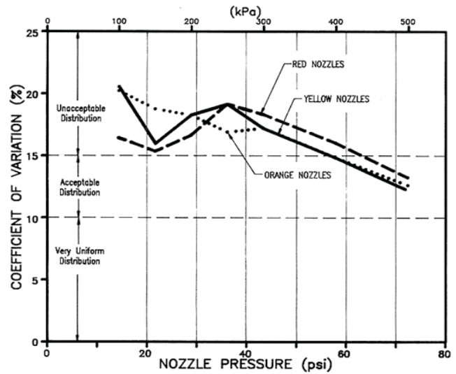
FIGURE 6. Spray Pattern Uniformity for Albus Yellow, Orange and Red 110 Degree Ceramic Nozzles Operated at a 15.7 in (400 mm) Nozzle Height.
