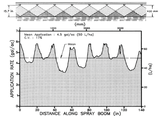
FIGURE 7. Typical Spray Distribution Pattern Along the Boom at a 44 psi (300 kPa) Nozzle Pressure Using Albus Red Ceramic Nozzles, at an 15.7 in (400 mm) Nozzle Height.
