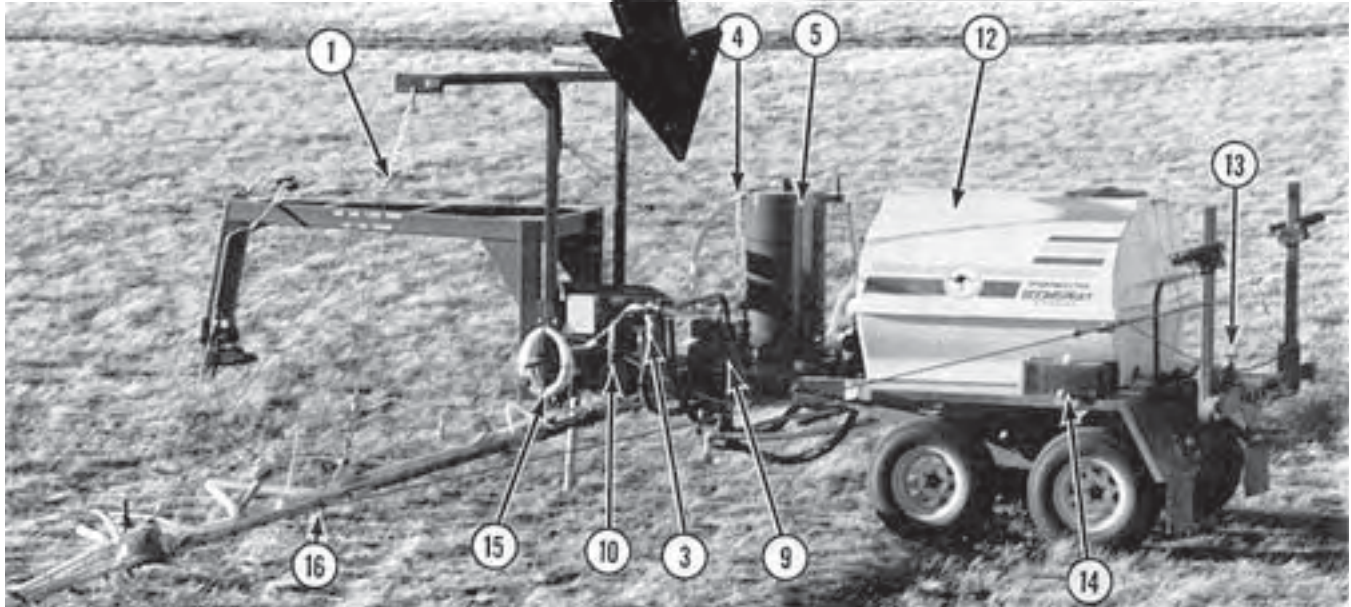
FIGURE 1. Spraymaster Model GN 40-60 Field Sprayer: (1) Boom Suspension Cables, (2) Flow and Pressure Sensors, (3) Main Valve, (4) Chemical Inductor Wand, (5) Foam Tank, (6) Agitator Valve, (7) Drain Valve, (8) Pump, (9) Motor and Compressor, (10) Self-Cleaning Line Strainer, (11) Motorized Control and Solenoid Valves, (12) Spray Tank, (13) Reload Hose, (14) Fresh Water Container, (15) Air Hose, (16) Spray Boom and Nozzle Body Assemblies.
