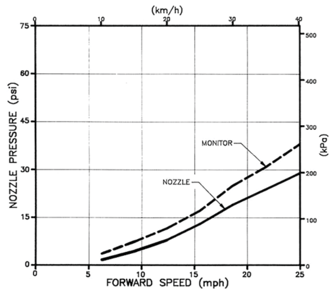
FIGURE 11. Actual Nozzle and Indicated Pressure Using Albus Red Nozzles at 4.5 gal/ac (50 L/ha).
