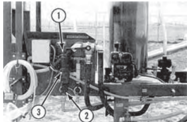
FIGURE 20. Line Strainer Plumbing Components: (1) Vent Caps, (2) Light Duty Valve, (3) Self-Cleaning Strainer.
