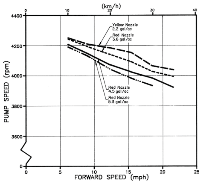
FIGURE 18. Pump Speed at Various Application Rates and Forward Speeds.
