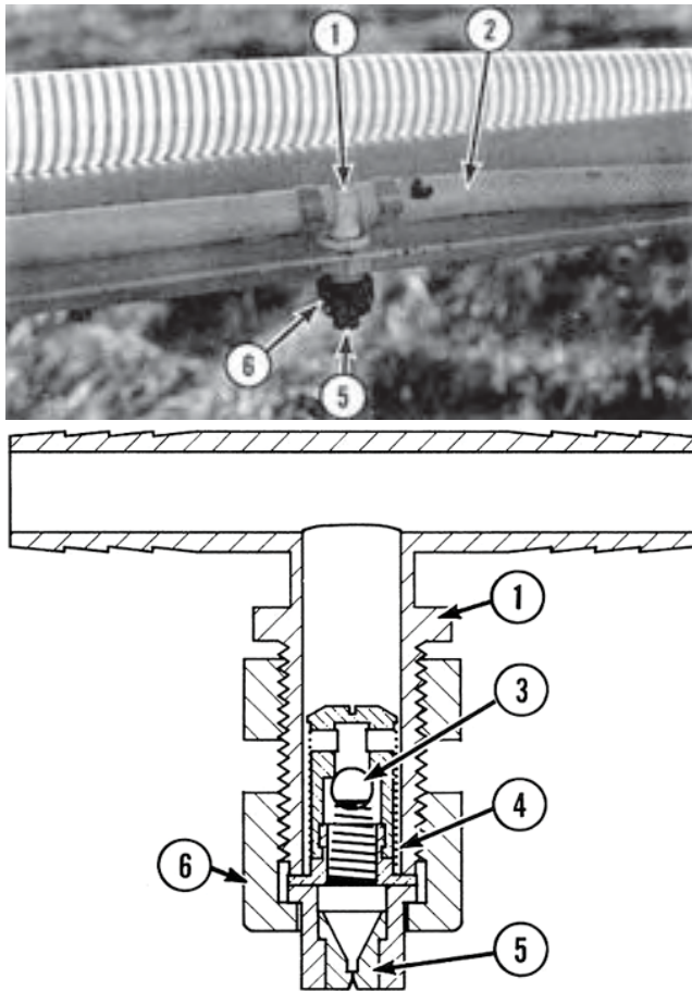
FIGURE 13. Hose Shank Nozzle Assembly: (1) Double Hose Connection (2) Spray Boom, (3) Check Valve, (4) Strainer, (5) Nozzle Tip, and (6) Threaded Nozzle Cap.
