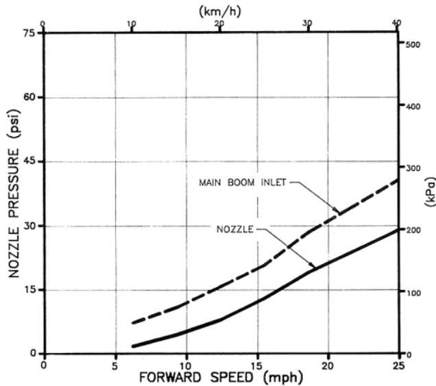
FIGURE 12. Pressure Loss From Boom Line Inlet to Nozzle Tip Using Albuz Red Nozzle Tips at 4.5 gal/ac (50 L/ha).
