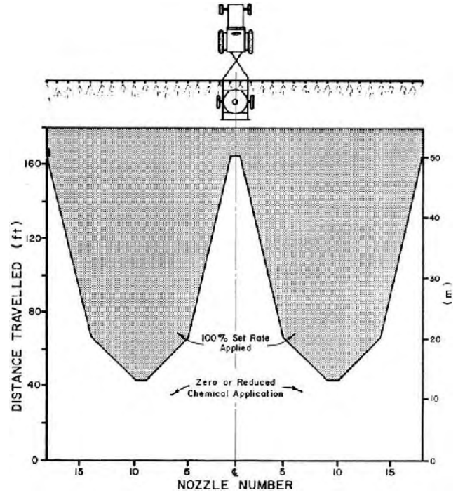
FIGURE 4. System Response Profile with 50 L/ha Spray Jets (Computerspray Jets #3).
