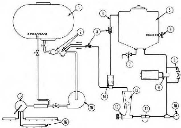
FIGURE 1. Schematic of Ag-Chemical Injector in a Sprayer Plumbing System: (1) Sprayer Water Tank, (2) Injection Manifold, (3) Check Valves, (4) Chemical Bypass, (5) Injector Chemical Tank, (6) Chemical Temperature Gauge, (7) Drain, (8) Chemical Pressure Control Valve, (9) Diaphragm Pump and 12 Volt Motor, (10) Chemical Pressure Gauge, (11) Filter, (12) Flow Meter, (13) Needle Valve Flow Control, (14) Solenoid Valve, (15) Sprayer Pump, (16) Sprayer Booms and Nozzles.
