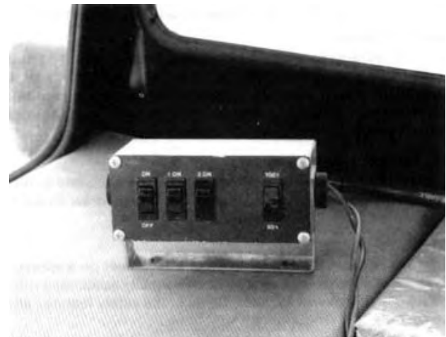
FIGURE 4. Remote Pump Control Box Mounted in Tractor Cab.
