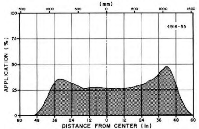
FIGURE 11. Effect of Flow Rates on Distribution Pattern with the Micromax Operated at Low Speed at an 18 in (457 mm) Discharge Height, 15 Degree Forward Angle and 21 psi (145 kPa) Pressure. (Upper: 4916-26, Lower: 4916-55).
