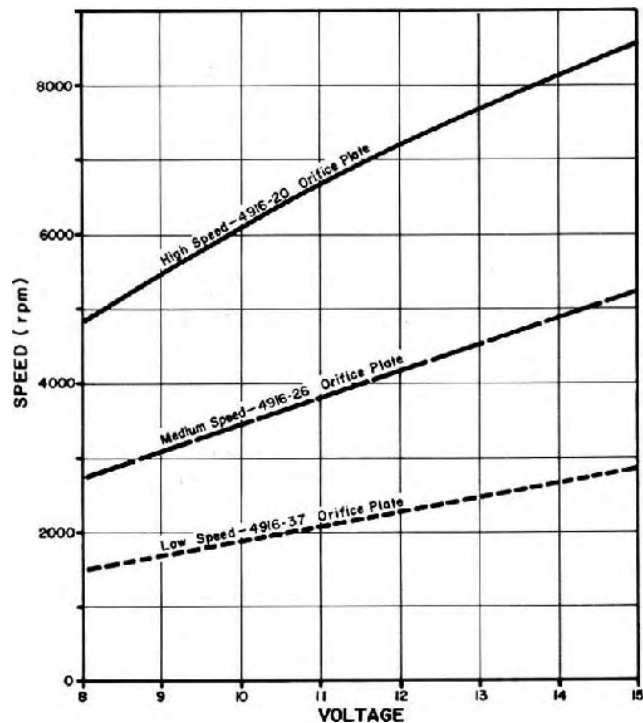
FIGURE 8. Micromax Spinning Disc Speeds at Various Supply Voltages at Low, Medium and High Speed Pulley Combinations.
