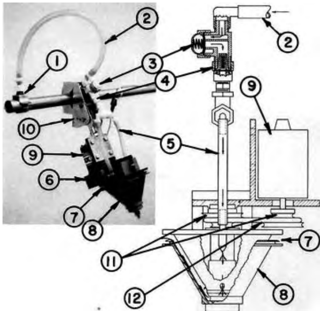
FIGURE 1. Micromax Controlled Droplet Applicator: (1) Existing Sprayer Nozzle Body, (2) Inlet Hose, (3) Diaphragm Check Valve, (4) Orifice Plate Adaptor, (5) Feeder Hoses, (6) Pulley Shield, (7) Spinning Disc Teeth, (8) Cone, (9) 12 Volt DC Motor, (10) Mounting Bracket, (11) Triple Pulley Assembly, (12) Belt.
