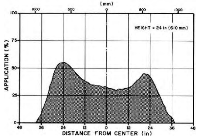
FIGURE 14. Effect of Applicator Height on Distribution Pattern, Operated at Low Speed at a 15 Degree Forward Angle and 21 psi (145 kPa) Pressure.
