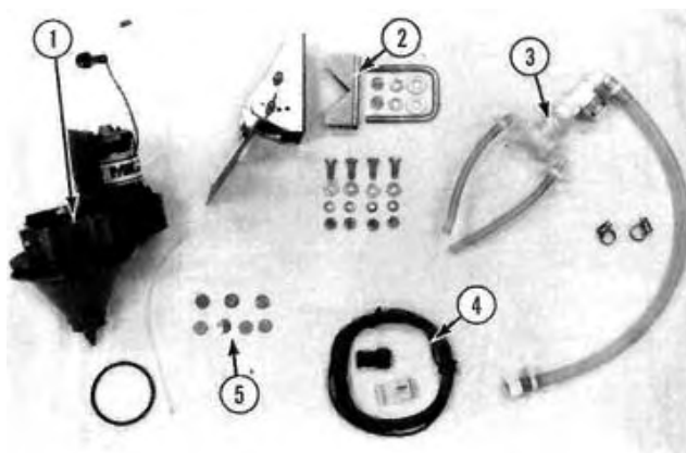
FIGURE 2. Micromax Applicator Parts: (1) Micromax Body and Motor, (2) Mounting Bracket and Hardware, (3) Plumbing Assembly, (4) Electrical Wire and Connectors, (5) Orifice Plates and Plugs.
