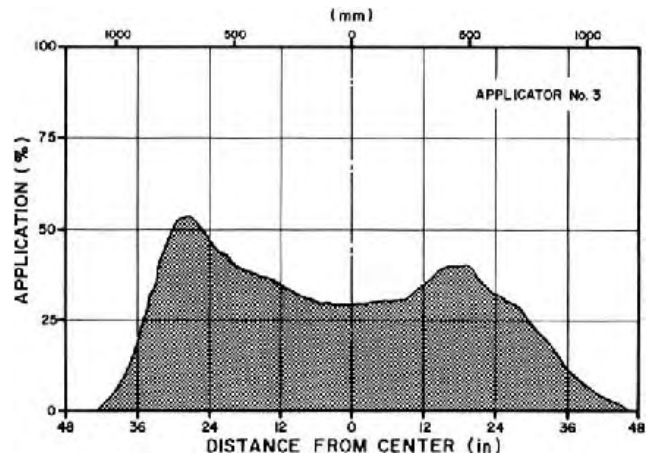
FIGURE 10. Distribution Patterns of Three Different Micromax Applicators Using 4916-37 Orifice Plates, Operated at Low Speed, at an 18 in (457 mm) Discharge Height, 15 Degree Forward Angle and 22 psi (150 kPa) Pressure.
