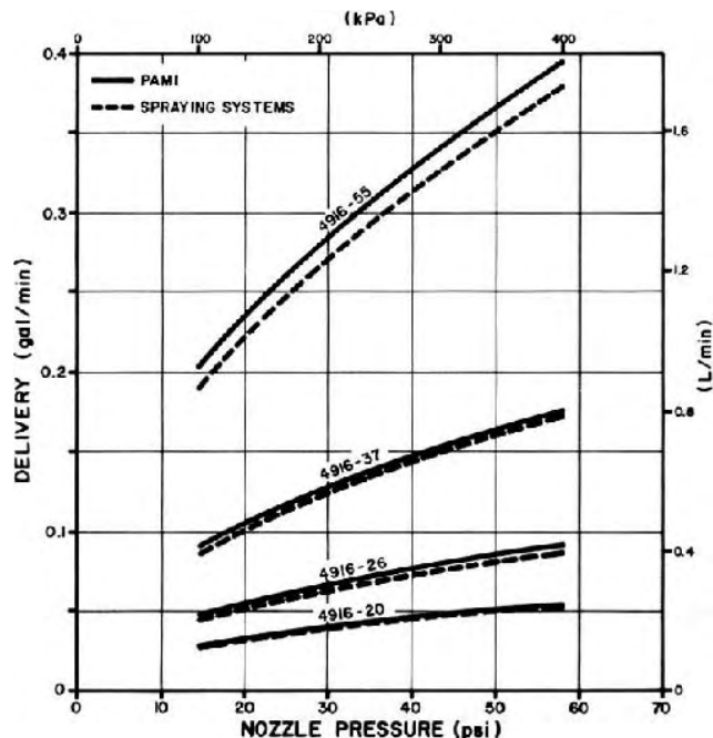
FIGURE 7. Delivery Rates for Stainless Steel Orifice Plates.
