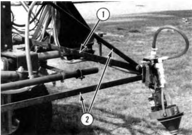
FIGURE 5. Micromax Applicator Mounted on Sprayer: (1) Extension Arms. (2) Bracing.
