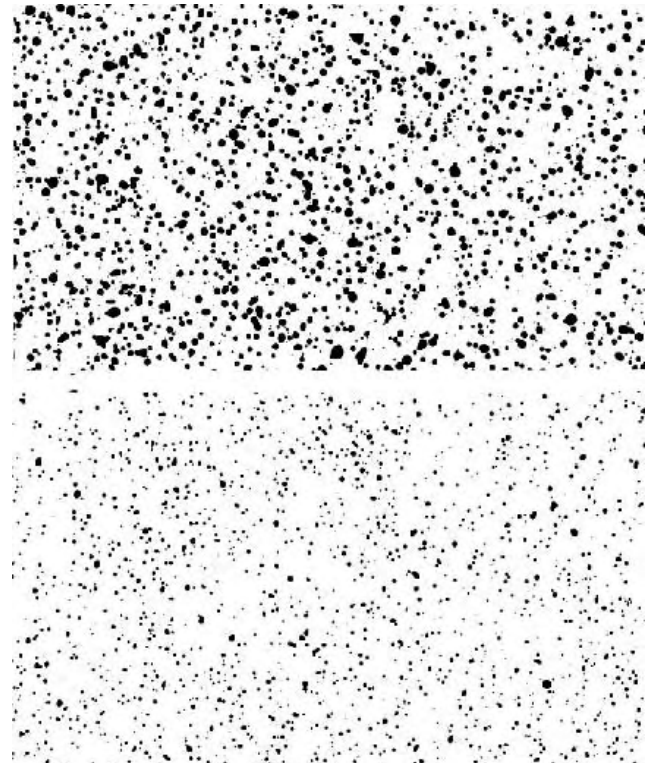
FIGURE 19. Droplet Sizes Produced by the Micromax when Spraying at the Low Speed (2465 rpm) (Upper: 4916-55 Orifice Plate, Lower: 4916-37 Orifice Plate).
