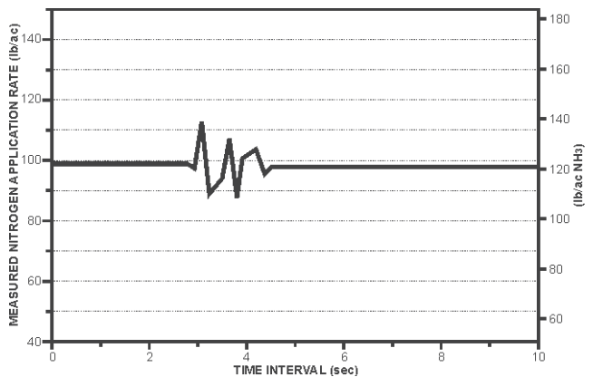
Figure 4. Controller response curve with a decrease in ground speed from 5 to 3 mph (8 to 4.8 km/h) at an application rate of 100 lb/ac (112 kg/ha).
