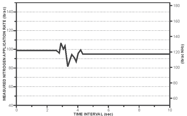
Figure 5. Controller response curve with an increase in ground speed from 5 to 7 mph (8 to 11.3 km/h) at an application rate of 100 lb/ac (112 kg/ac).
