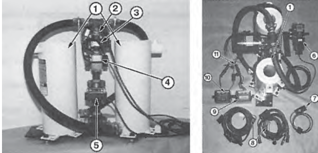
Figure 2. DICKEY-john NH 3 Control System: (1) Thermal Transfer Unit, (2) Actuator Assembly, (3) Motorized Control Valve, (4) Vapour Detector, (5) Flow Meter, (6) Radar II Speed Sensor, (7) Off/Auto/Flush Switch, (8) Electrical Cables, (9) Control Console, (10) Monitor Console and (11) Y-Cable.
