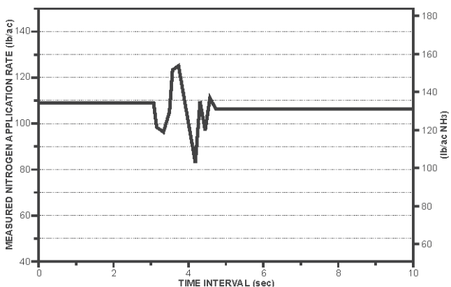
Figure 5. Controller response curve with a decrease in ground speed from 5 to 3 mph (8 to 5 km/h) at an application rate of 100 lb/ac (112 kg/ha).
