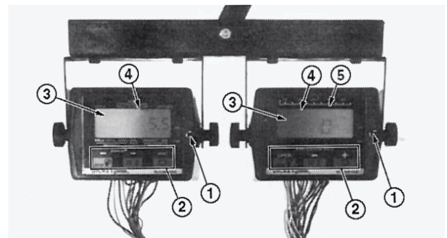
Figure 8. LEFT: DICKEY-john DjCMS100 Monitor Console: (1) power switch, (2) function keypad, (3) data display screen and (4) function's pointer. RIGHT: DICKEY-john DjCCS100 Control Console: (1) power switch, (2) function keypads, (3) data display screen, (4) bar graph display and (5) setup position location.
