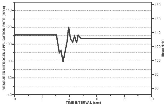
Figure 6. Controller response curve with an increase in ground speed from 5 to 7 mph (8 to 12 km/h) at an application rate of 100 lb/ac (112 kg/ha).
