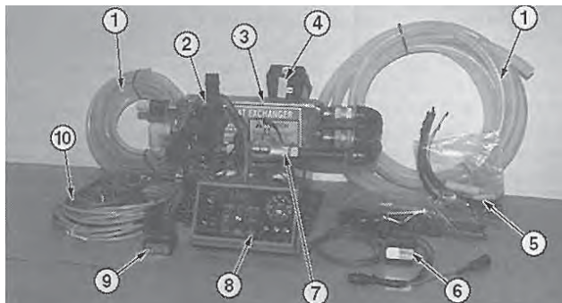
Figure 2. Micro-Trak MT3000 NH 3 Control System: (1) Vapour Hoses, (2) Motorized Control Servo Valve, (3) Heat Exchanger, (4) On/Off Valve, (5) Mounting Hardware, (6) Radar Interface Cable and Module, (7) Flow Meter, (8) Control Console, (9) Hold Cutout Module and (10) Electrical Cables.
