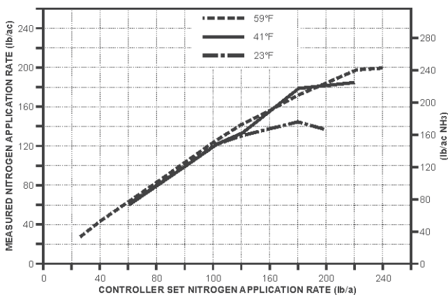
Figure 3. Measured nitrogen application rates.
