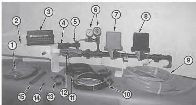
Figure 2. Raven SCS440 Anhydrous Ammonia Control System: (1) Mounting Hardware, (2) Heat Exchanger, (3) Control Console, (4) Strainer Assembly, (5) Emergency Shut-off Valve, (6) Pressure and Temperature Gauges, (7) Motorized Control Valve, (8) On/Off Valve, (9) Vapour Hoses, (10) Console Control Cable, (11) Flow/Meter Cable, (12) Flow Meter (13) Radar Interface Cable, (14) Motorized Control Valve Reversing Cable and (15) Steel Vapour Tubes.
