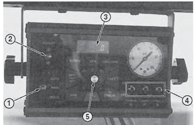
Figure 9. Micro-Trak MT3000 Control Console: (1) Master Spray Switch, (2) Adjust Switch, (3) Data Display Screen, (4) Boom Switches and (5) Rotary Selector Dial.
