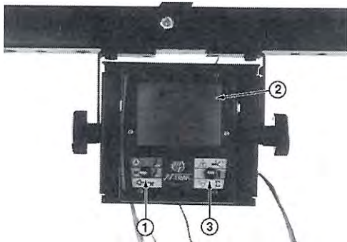
Figure 8. Nitro-Trak TNc9541 Display Console: (1) Master Switch, (2) Data Display Screen and (3) Rate Switch.
