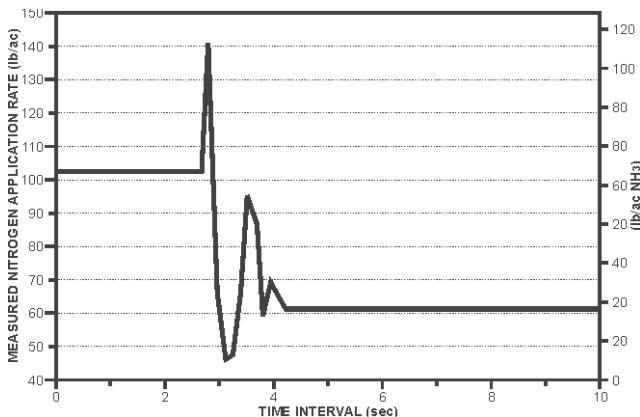
Figure 6. Controller response curve with a decrease in application rate from 100 to 60 lb/ac (112 to 67 kg/ha) at a ground speed of 5 mph (8 km/h).
