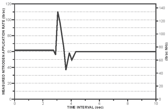
Figure 5. Controller response curve with a decrease in ground speed from 5 to 3 mph (8 to 4.8 km/h) at an application rate of 60 lb/ac (67 kg/ha).
