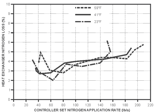
Figure 4. Percentage of nitrogen loss from the vapour lines.
