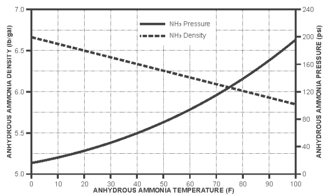
Figure 1. NH 3 physical properties.
