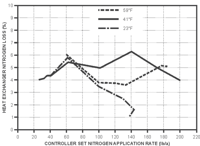
Figure 4. Percentage of nitrogen discharged from the vapour lines.
