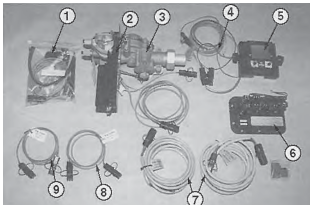
Figure 2. Nitro-Trak NH 3 Automatic Control System: (1) Magnetic Speed Sensor Kit, (2) B-9500 Meter Control Kit, (3) Continental B-9500 Meter, (4) Power Cable, (5) TNc9541 Display Console, (6) TNsc942 Servo Control Module, (7) Extension Cables, (8) Run/Hold Cable and (9) Temperature Cable.
