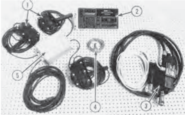
FIGURE 1. Senstek DCM-2 Depth Control System: (1) Sensor, (2) Control Console, (3) Electro-hydraulic Solenoid Valve, (4) Temperature Sensor, (5) Implement Module.
