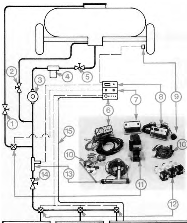
FIGURE 1. SED Automatic Sprayer Control System: (1) By-Pass Valve, (2) Agitator Valve, (3) Pump, (4) Filter, (5) Shut-Off Valve, (6) Model 944 Remote Control, (7) Model 948 Automatic Rate Controller, (8) Model 943A Sprayer Monitor, (9) Speed Sensor, (10) Cables with Puli-Apart Connectors, (11) Motorized Control Valve, (12) Solenoid Valves, (13) Flow Sensor, (14) Throttling Valve, (15) Boom Pressure Line.
