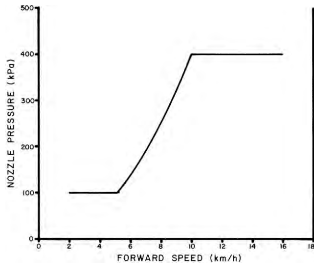
FIGURE 7. Nozzle Pressure at Various Forward Speeds with the Automatic Sprayer Control System with an Increased Preset Pressure Range.
