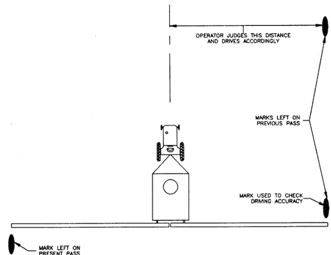
FIGURE 4. Schematic Illustrating Peacock Foam Marker Operation.
