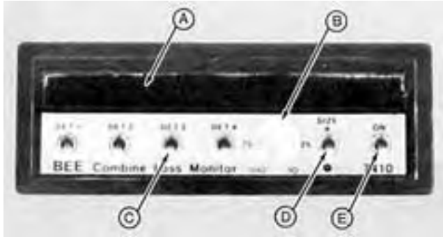
FIGURE 3. Control Box: (A) Loss Indicator (B) Calibration Control (C) Sensor Selectors (D) Sensitivity Control (E) Power Switch.
