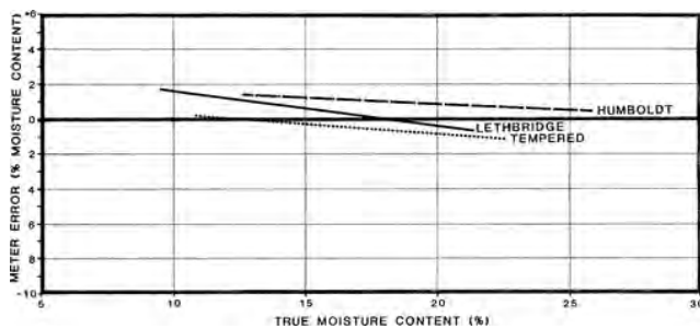
Figure 6. Deviations of Meter Readings for Dickey-john in Three different Types of Spring Wheat.
