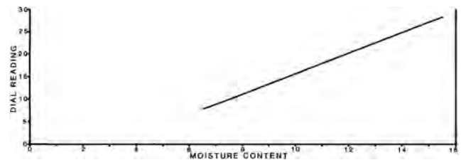
Figure 5. Calibration Curve for Dickey-john in Rapeseed.
