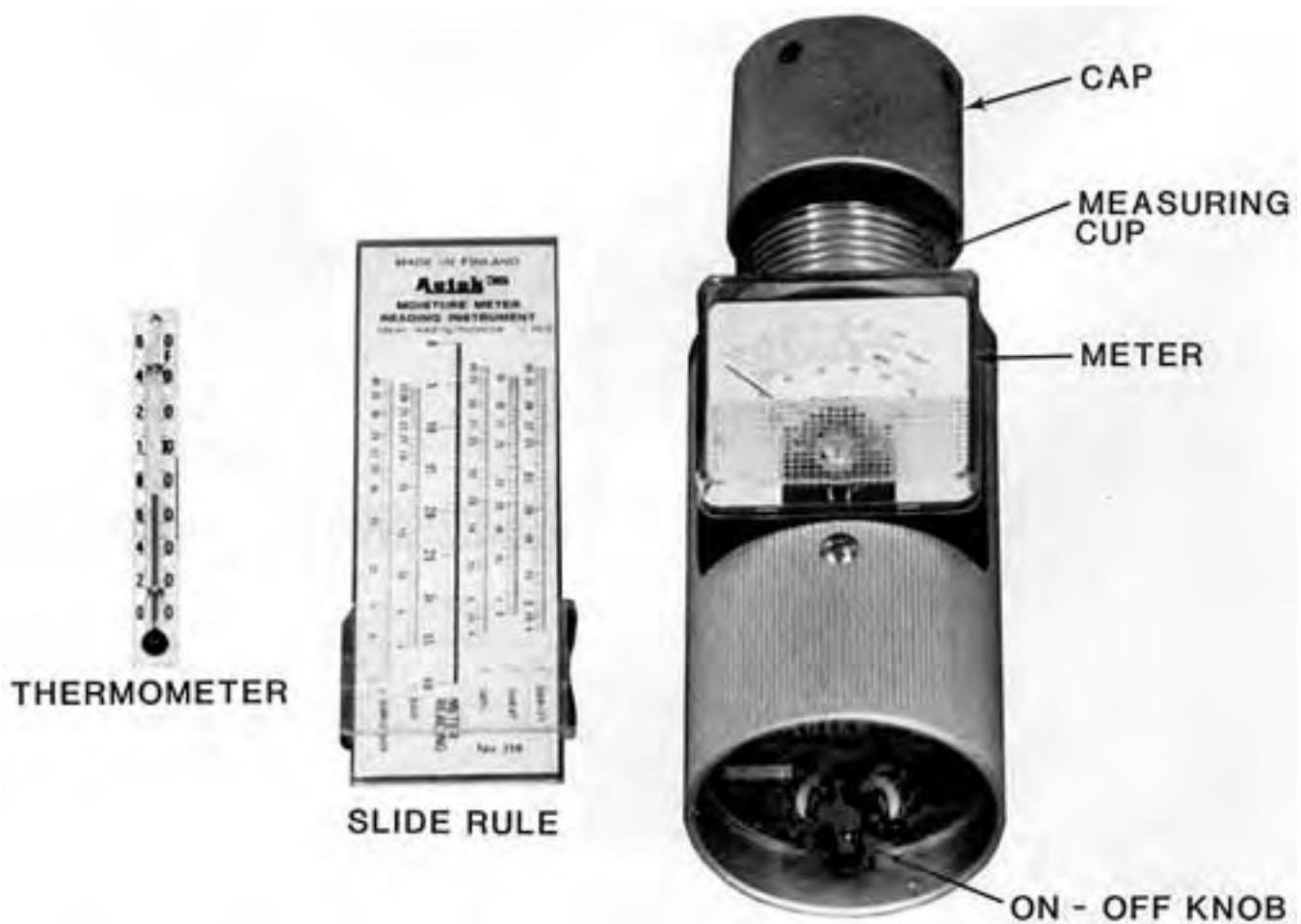
Figure 1. Detailed View of Agtek-35 Grain Moisture Meter.
