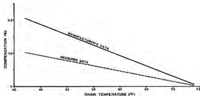
Figure 8. Errors in Temperature Compensation at Varying Grain Temperatures with the Agtek Meter at 23°C (74°F).
