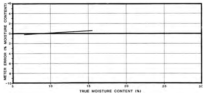
Figure 6. Deviations of Meter Readings for Agtek-35 in Rapeseed.
