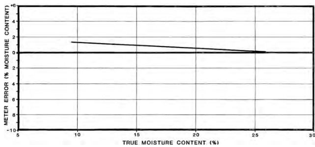
Figure 3. Deviations of Meter Readings for Agtek-35 in Wheat.
