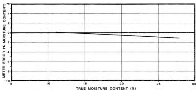
Figure 5. Deviations of Meter Readings for Agtek-35 in Oats.
