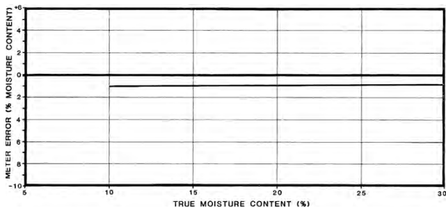
Figure 4. Deviations of Meter Readings for Agtek-35 in Barley.
