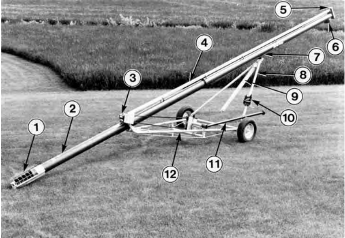
FIGURE 1. Farm King 8 x 41 Grain Auger: (1) Inlet, (2) Auger Tube, (3) Gear Box, (4) Drive Shaft, (5) Upper End Drive, (6) Discharge Spout, (7) Elevating Track, (8) Lift Arms, (9) Telescoping Mast, (10) Cable Winch, (11) Power Take-off Drive Line, (12) Lower Arms.
