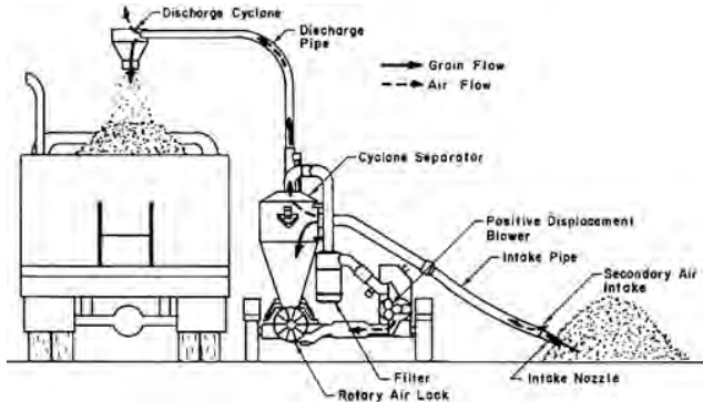
FIGURE 1. Schematic View Showing Air and Grain Flow.
