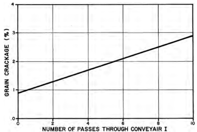
FIGURE 14. Grain Crackage in Dry Wheat.
