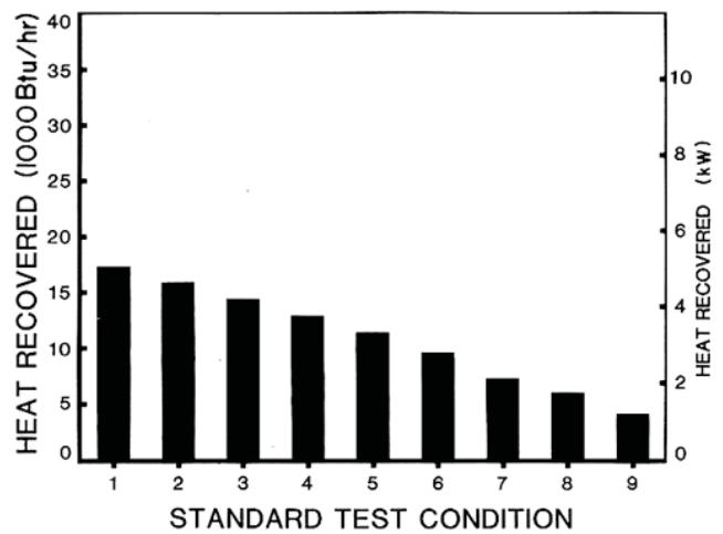
FIGURE 7. Average Heat Recovery of the Del-Air A350.
