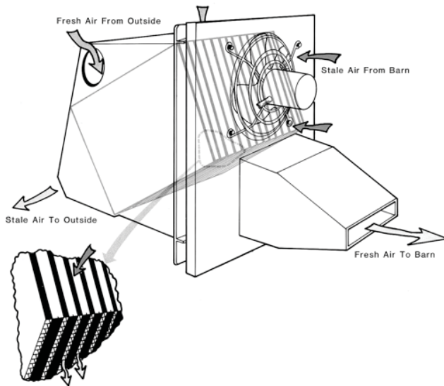
FIGURE 1. Del-Air A350 Heat Exchanger.
