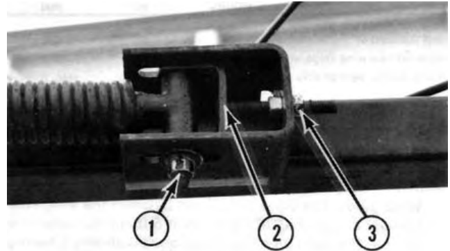
FIGURE 7. Harrow Tine Adjustment: (1) Carriage Bolt, (2) Adjusting Clevis, (3) Nuts.
