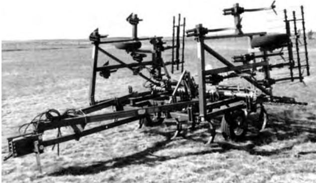
FIGURE 6. Transport Position.
