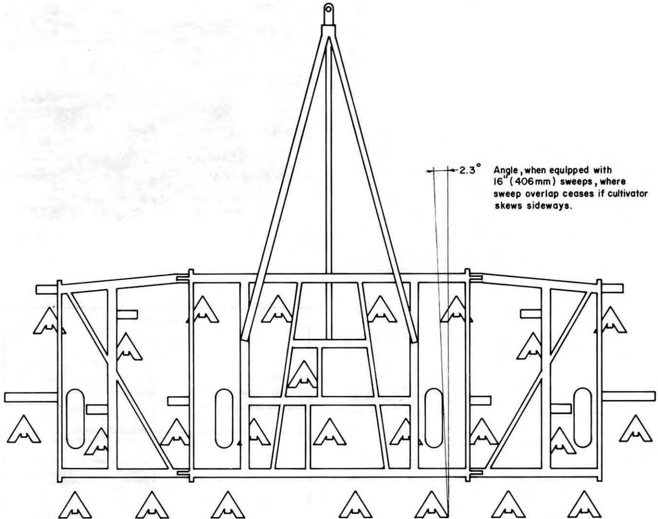
FIGURE 5. Sweep Pattern.
