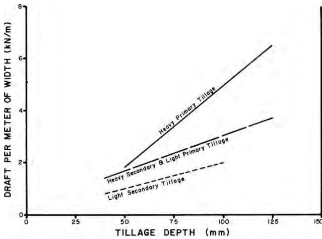
FIGURE 11. Average Draft Requirements for Cultivators at 8 km/h
