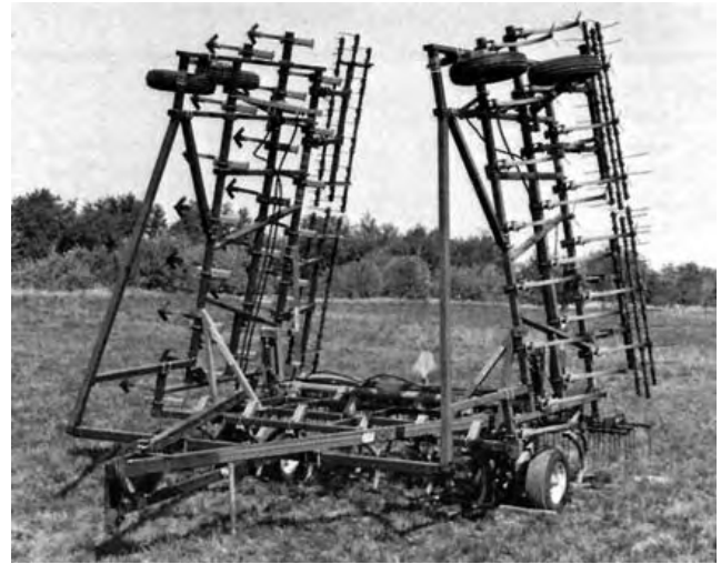
FIGURE 7. Transport Position.
