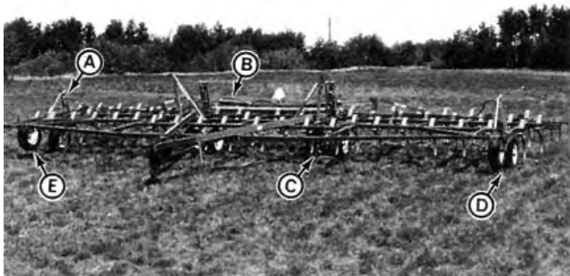
FIGURE 1. CI 279: (A) Depth Control Cylinders, (B) Wing Lift Cylinders, (C) Centre Wheels, (D) Wing Wheels, (E) Stabilizer Wheels.
