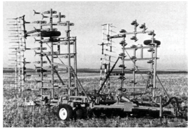
FIGURE 7. Transport Position.
