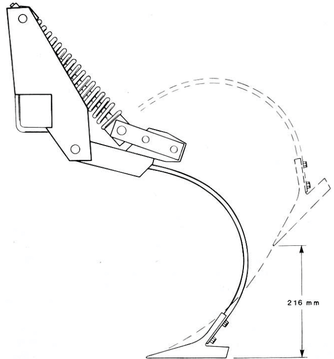
FIGURE 4. Shank Lifting Pattern (Spring Clamp In Normal Position).
