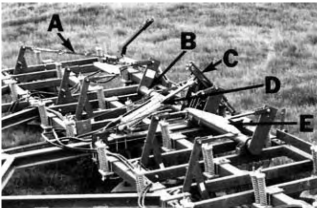
FIGURE 10. Depth Control Linkages: (A) Wing Cable, (B) Mainframe Rockshaft, (C) Depth Control Bars, (D) Master Cylinder, (E) Equalizer Bar.
