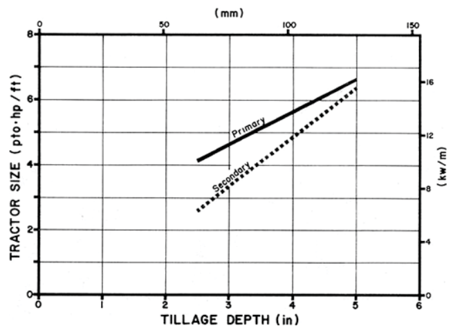
FIGURE 14. Average Horsepower Requirements for Blade Plows at 5 mph (8 km/h).
