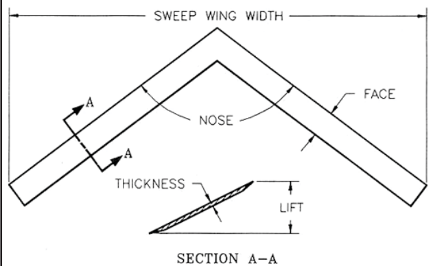
FIGURE 17. Sweep Terminology
