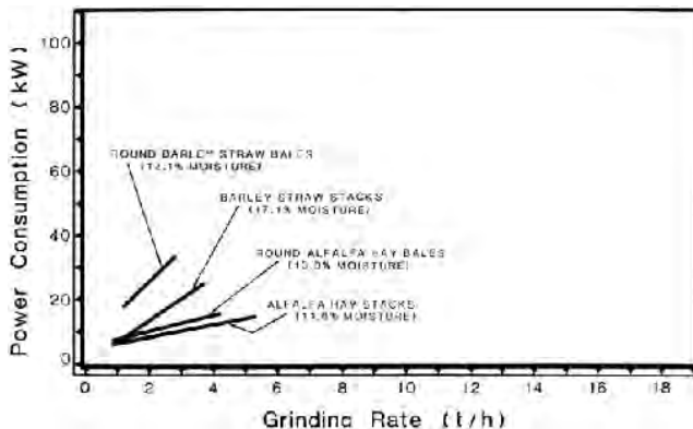
FIGURE 7. Power Consumption of the Farmhand F890-A, at Various Grinding Rates, when Equipped with a 51 mm (2 in) Screen.
