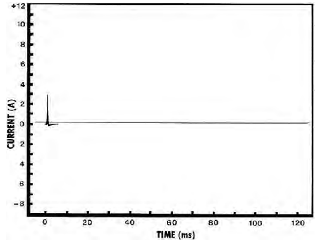
FIGURE 4. Current Delivered to a Well-Insulated Cow Touching a 16 km Well-Insulated Fence.
