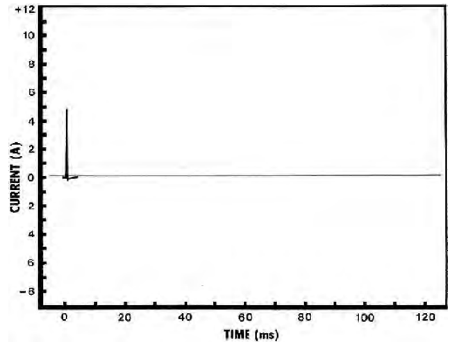
FIGURE 3. Current Delivered to a Well-Insulated Cow Touching a 5.4 km Well-Insulated Fence.
