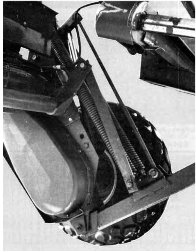
FIGURE 14. Table Floatation System.
