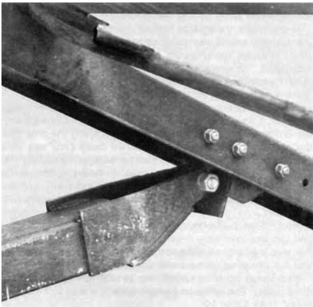
FIGURE 15. Lift Support Arms.
