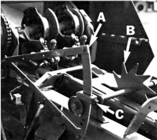
FIGURE 4. Bale Length Adjustment: (A) Metering Arm, (B) Metering Wheel, (C) Adjustable Stop.
