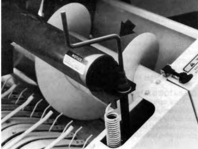
FIGURE 7. Pickup Height Adjustment.
