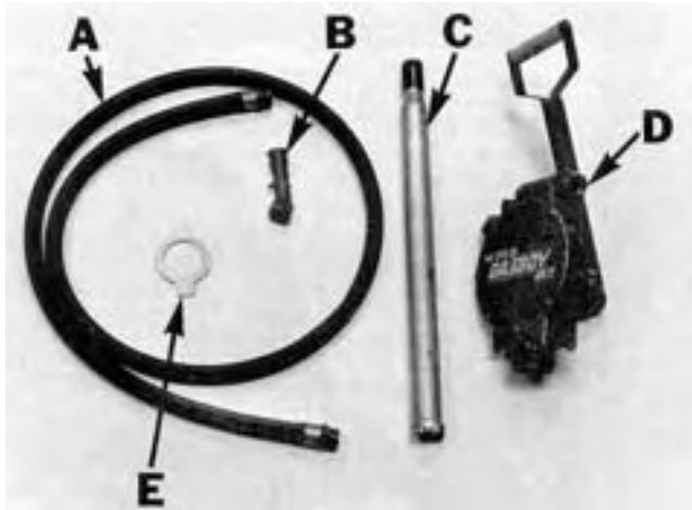
FIGURE 1. Gasboy Superjet Model 1720 Hand Pump: (A) Outlet Hose, (B) Outlet Nozzle (C) Telescopic Suction Pipe, (D) Pump Body, (E) Lock Collar.
