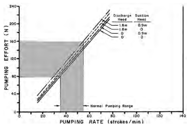
FIGURE 3. Pumping Effort with Diesel Fuel at Various Pumping Rates, Suction and Discharge Heads.
