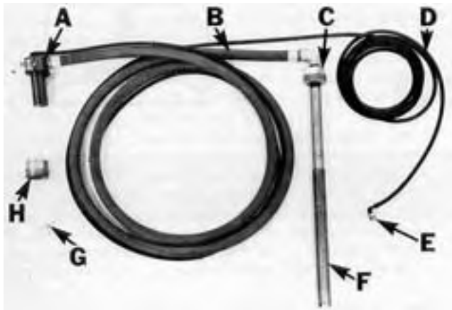
FIGURE 1. Vac-U-Fil Fuel Transfer Pump: (A) Pump Body, (B) Fuel Transfer Hose, (C) Bung Adaptor, (D) Vacuum Hose, (E) Manifold Adaptor, (F) Telescoping Suction Pipe, (G) 3 Way Barbed Tee, (H) Storage Adaptor.
