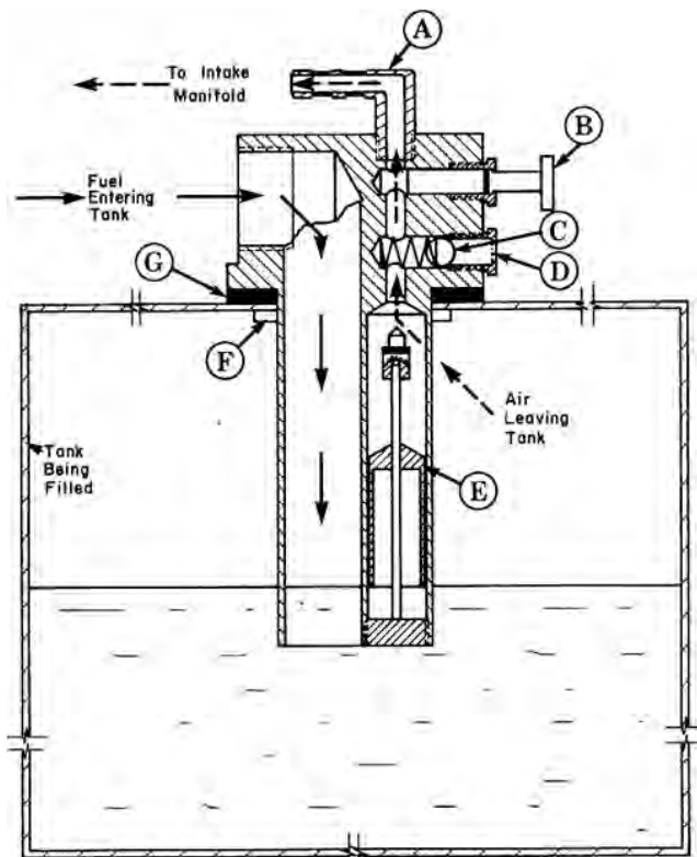
FIGURE 2. Schematic View of Vac-U-Fil Fuel Transfer Pump: (A) 90° Elbow, (B) Control Valve, (C) Relief Valve, (D) Screen, (E) Float Valve, (F) Locking Pins, (G) Gasket
