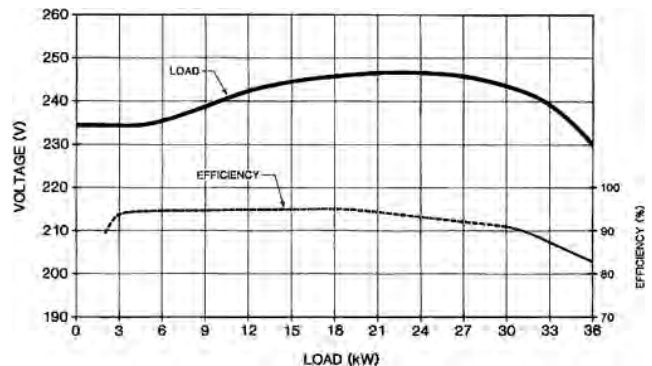
FIGURE 2. Performance characteristics.
