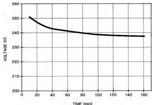
FIGURE 3. Endurance Test.
