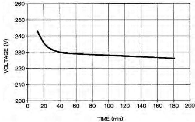
FIGURE 3. Endurance Test.
