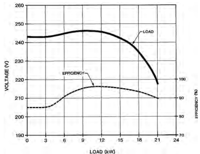
FIGURE 2. Performance characteristics.
