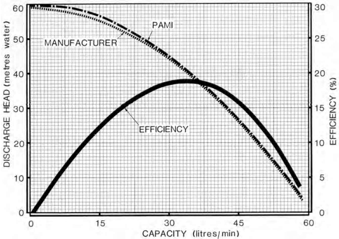
FIGURE 1. Performance Characteristics
